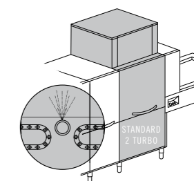
DRF99MB2 + 900 mm 16,1 kW Stage dryer with blowers and double belt
